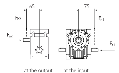
Bearing forces
