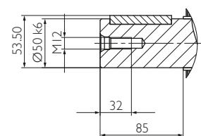
Detail I
