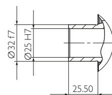
Detail I
