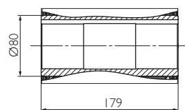
Detail I
